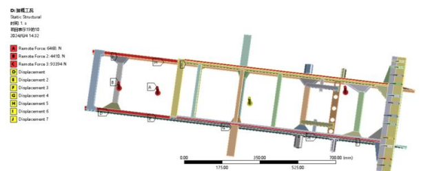
Figure 12 Load and constraints of the original chassis under unloading conditions
